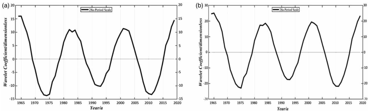
Figure 6 | Real part process of wavelet under the characteristic time scale of the first main period. (a) Gaju (b) Yunjinghong.
