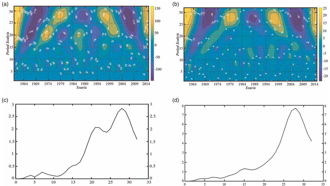
Figure 5 | (a,b) Contour maps of wavelet coefficients for the real parts at Gaju and Yunjinghong stations. (c,d) Graphs of wavelet variance at Gaju and Yunjinghong stations.
