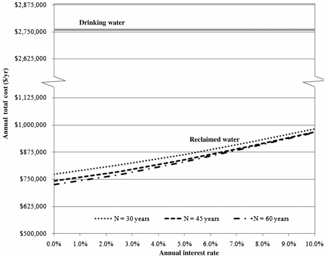
Figure 5 | Total annual costs for drinking water exceed those for reclaimed water over a range of annual interest rates and amortization periods, making reclaimed water use for non-potable purposes economically feasible.
