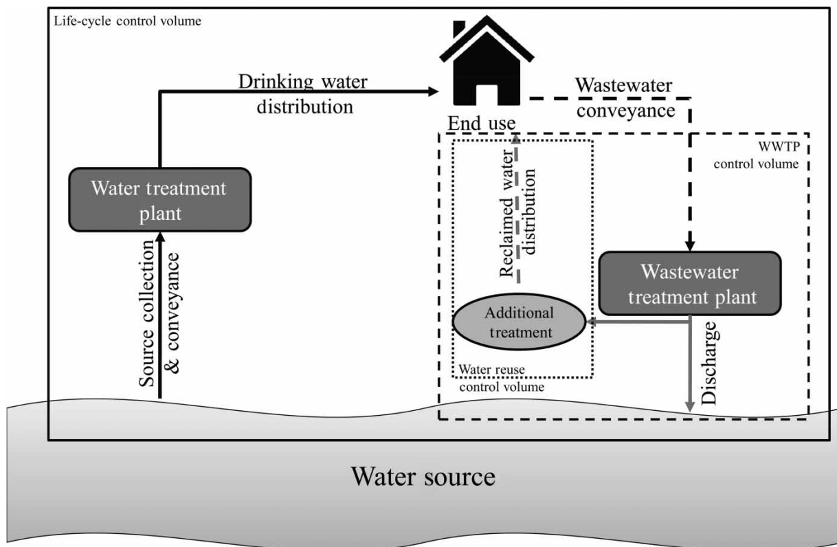
Figure 2 | Accounting for energy use for reclaimed water depends on how the control volume boundary is drawn. When considering the life-cycle control volume (solid line), energy use includes that associated with drinking water, wastewater treatment, and reclaimed water distribution. The wastewater treatment plant (WWTP) control volume (dashed line) includes energy consumption for wastewater treatment and reclaimed water distribution. The water reuse control volume (dotted line) includes only additional treatment (if necessary) and reclaimed water distribution.
