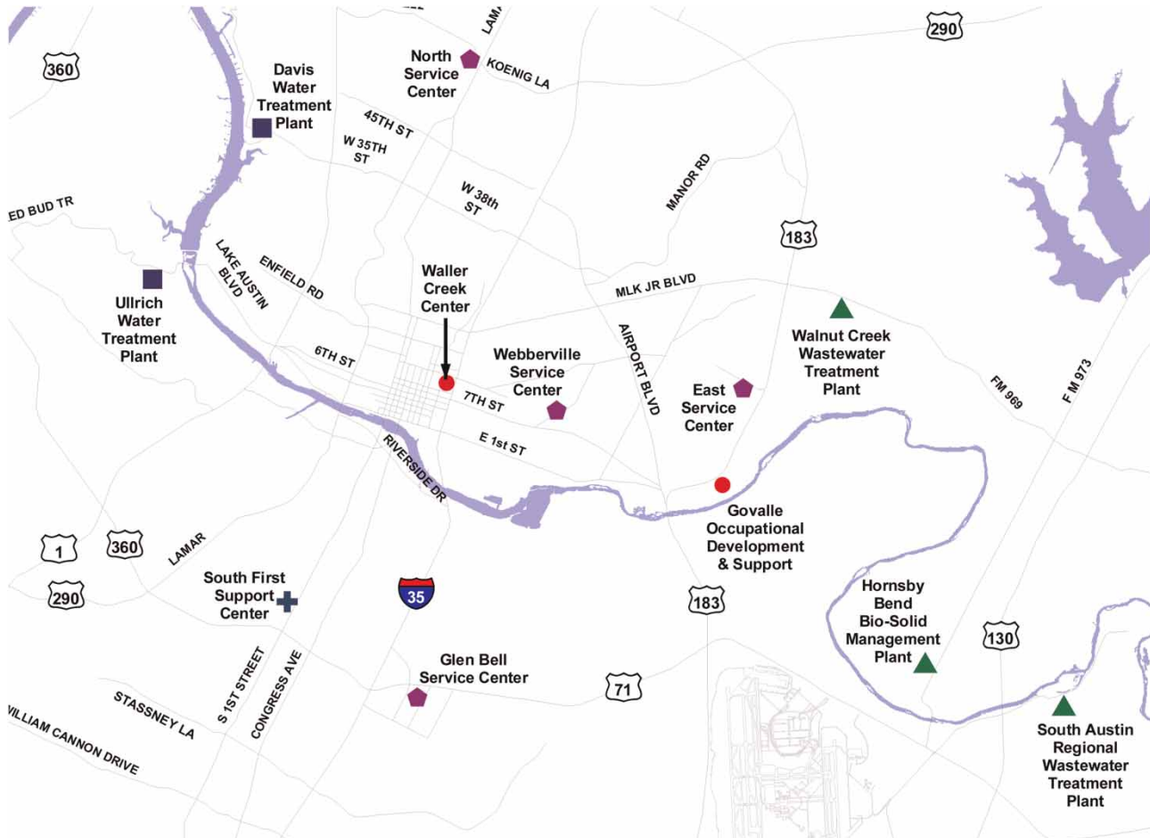
Figure 3 | Water (squares) and wastewater (triangles) treatment facilities are located on the west (higher elevation) and east (lower elevation) sides, respectively, of the Austin core.
